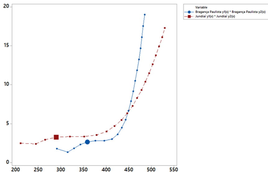
Fig. 7. Pareto frontiers for Braganca Paulista-SP and Jundiai-SP.
