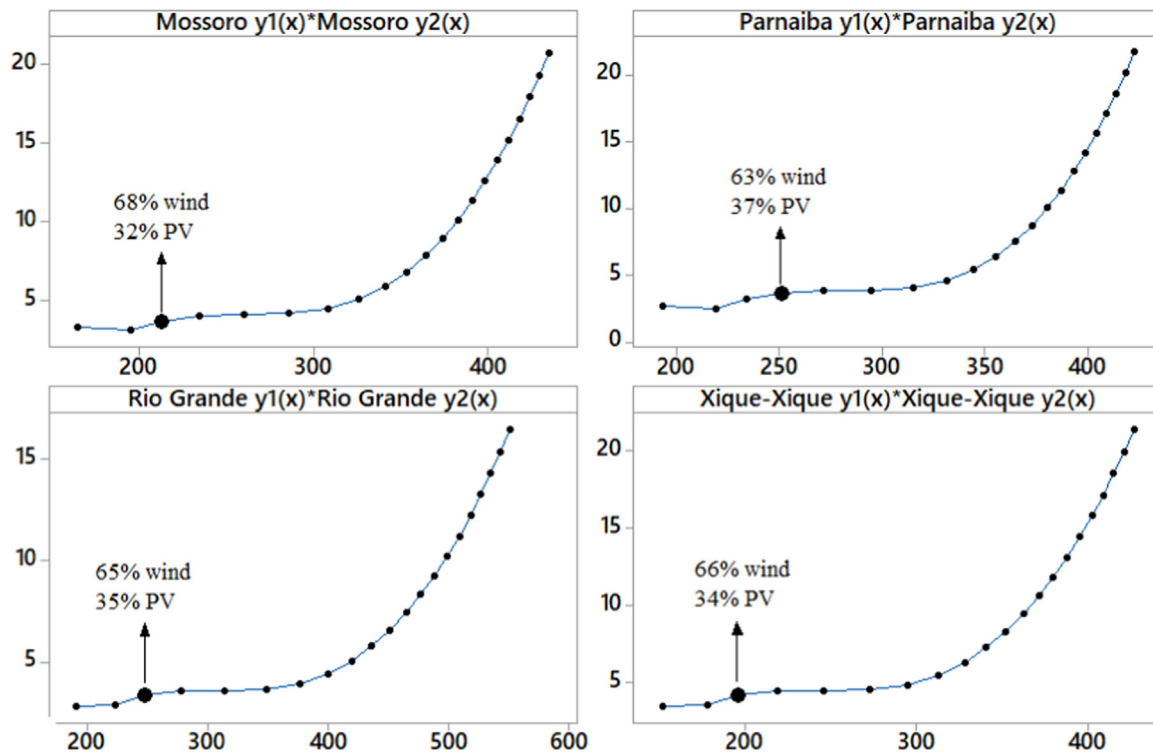
Fig. 5. Pareto frontier and optimal configuration in Mossoro, Parnaíba, Rio Grande, and Xique-Xique.
