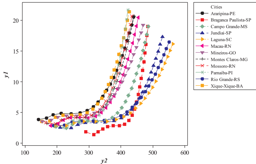
Fig. 6. Pareto frontiers of all analyzed cities.
